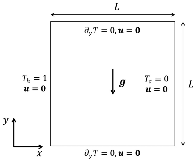
FIG. 12. Configuration of the 2D natural convection problem.
