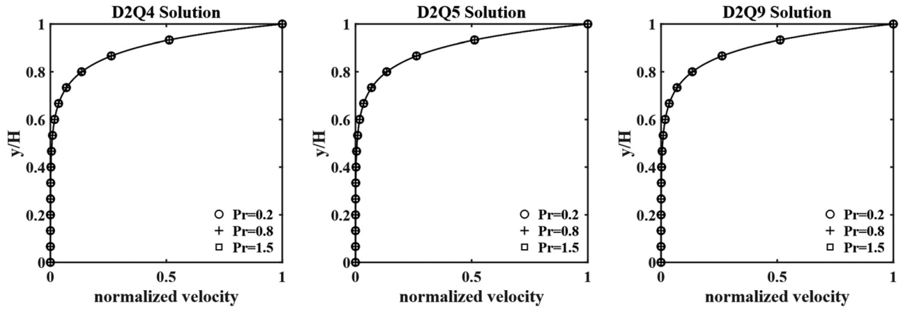
FIG. 10. Distributions of the normalized velocity u/u_0 along the vertical centerline with the D2Q4 model (left), the D2Q5 model (middle) and the D2Q9 model (right) at Re = 10 , Pr = [0.2, 0.8, 1.5] . The black solid lines “—” represent the analytical solution.
