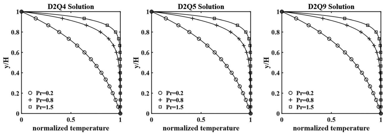
FIG. 11. Distributions of the normalized temperature (T - T_c)/\Delta T along the vertical centerline with the D2Q4 model (left), the D2Q5 model (middle) and the D2Q9 model (right) at Re = 10 , Pr = [0.2, 0.8, 1.5] . The black solid lines “—” represent the analytical solution.
