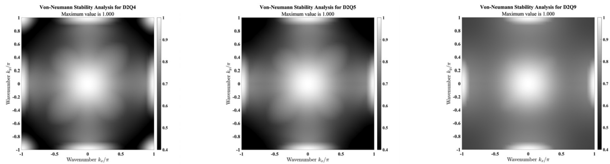
(b) Stability analysis for D2Q4 (left), D2Q5 (middle) and D2Q9 (right) with the mean flow velocity |u| = 0.15
