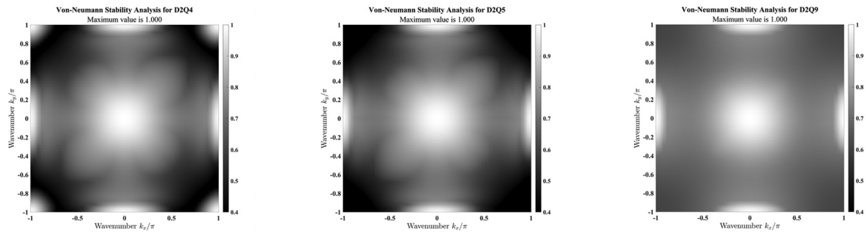
(c) Stability analysis for D2Q4 (left), D2Q5 (middle) and D2Q9 (right) with the mean flow velocity |u| = 0.20
