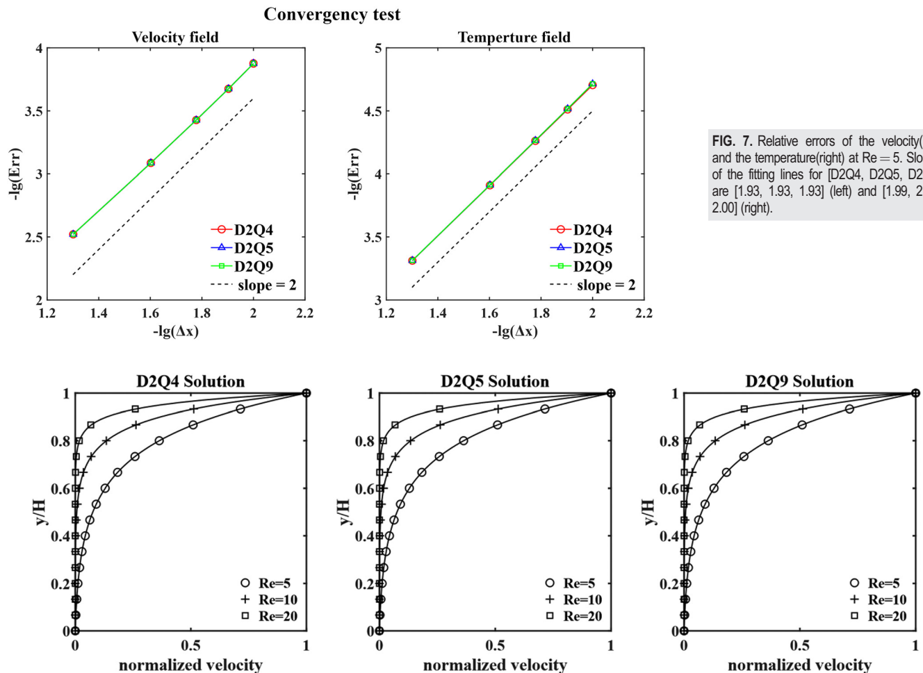
FIG. 8. Distributions of the normalized velocity u/u_0 along the vertical centerline with the D2Q4 model (left), the D2Q5 model (middle), and the D2Q9 model (right) at Pr = 0.71 , Re = [5, 10, 20] . The black solid lines represent the analytical solution.
