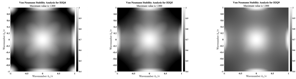
(a) Stability analysis for D2Q4 (left), D2Q5 (middle) and D2Q9 (right) with the mean flow velocity |u| = 0.10
