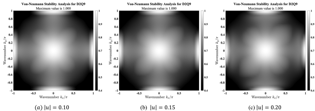
FIG. 3. Maximum eigenvalue magnitude of the SLBM as a function of wavenumber vector under a different mean flow velocity |u| for \tau_v = 0.5 .
