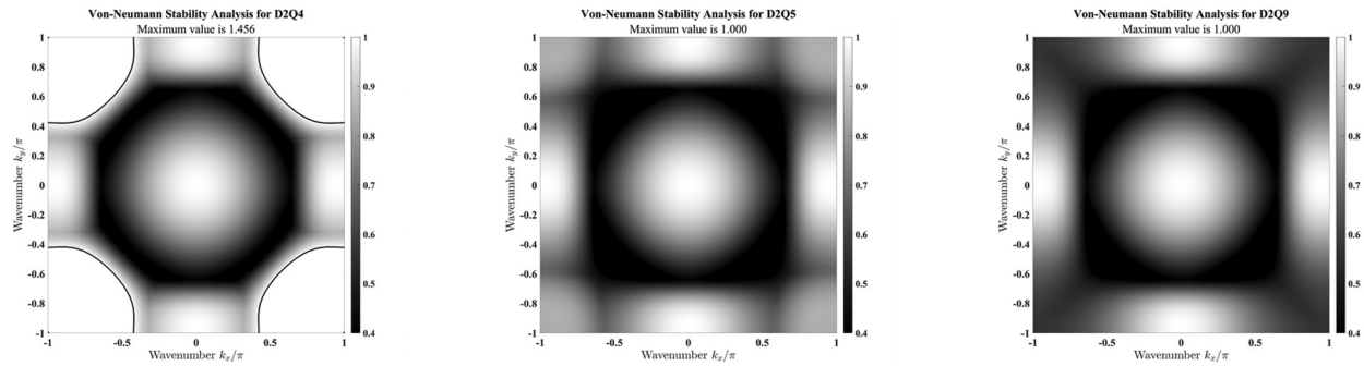
(a) Stability analysis of the STLBM with the D2Q4 (left), the D2Q5 (middle) and the D2Q9 (right) thermal lattice velocity models on the mesh size of 301 \times 301 .
