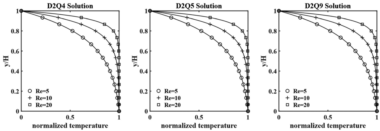
FIG. 9. Distributions of the normalized temperature (T - T_c)/\Delta T along the vertical centerline with the D2Q4 model (left), the D2Q5 model (middle), and the D2Q9 model (right) at Pr = 0.71 , Re = [5, 10, 20] . The black solid lines “—” represent the analytical solution.
