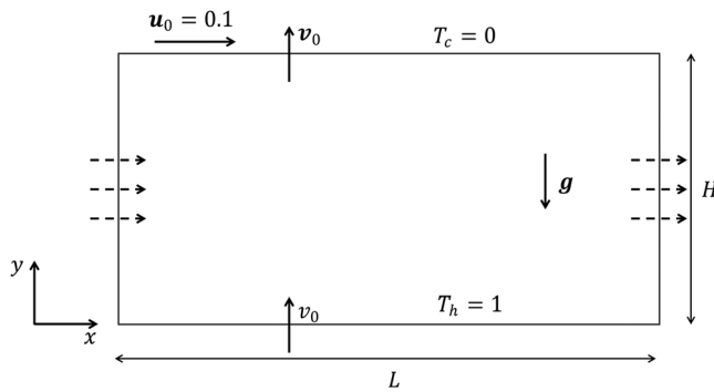
FIG. 6. Configuration of the porous plate problem.
