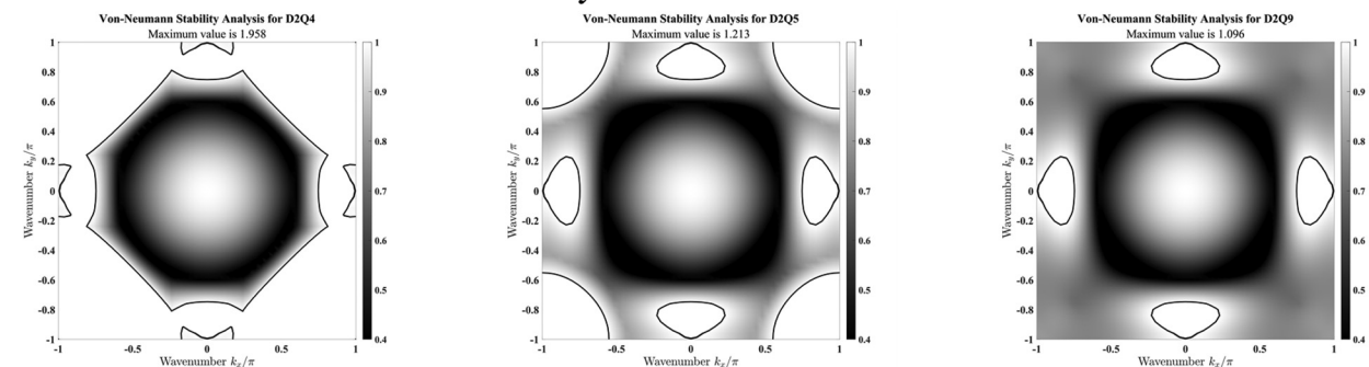
(c) Stability analysis of the STLBM with the D2Q4 (left), the D2Q5 (middle) and the D2Q9 (right) thermal lattice velocity models on the mesh size of 401 \times 401 .
