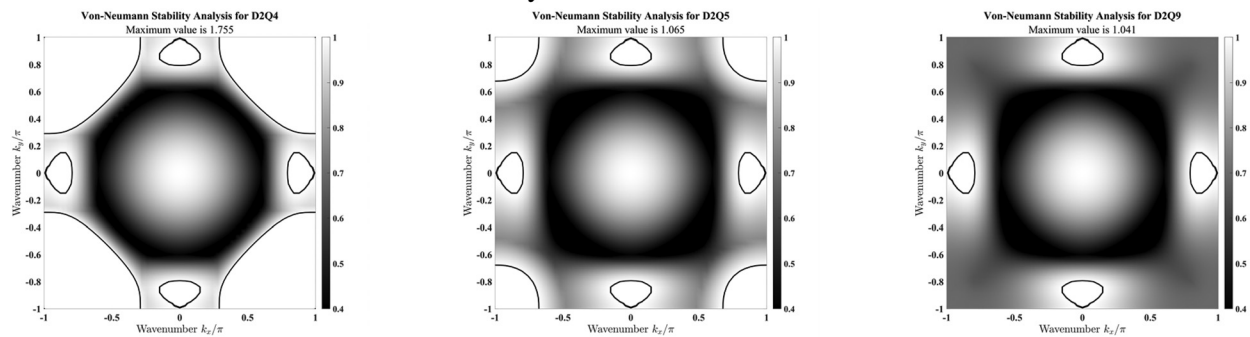
(b) Stability analysis of the STLBM with the D2Q4 (left), the D2Q5 (middle) and the D2Q9 (right) thermal lattice velocity models on the mesh size of 361 \times 361 .
